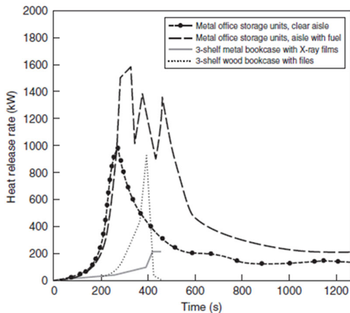
Figure 3-1.13. Storage units.
